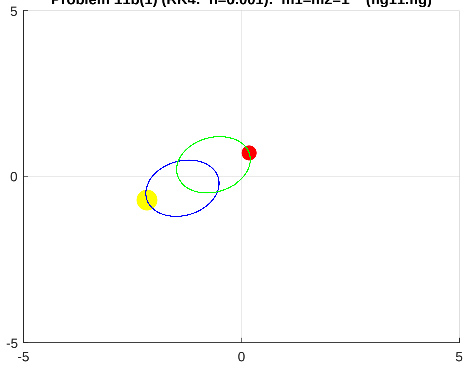
Celestial Mechanics: Two (2) Body Problem Problem 11b(1) (RK4: h=0.001 ): m_1=m_2=1 (fig11.fig)
